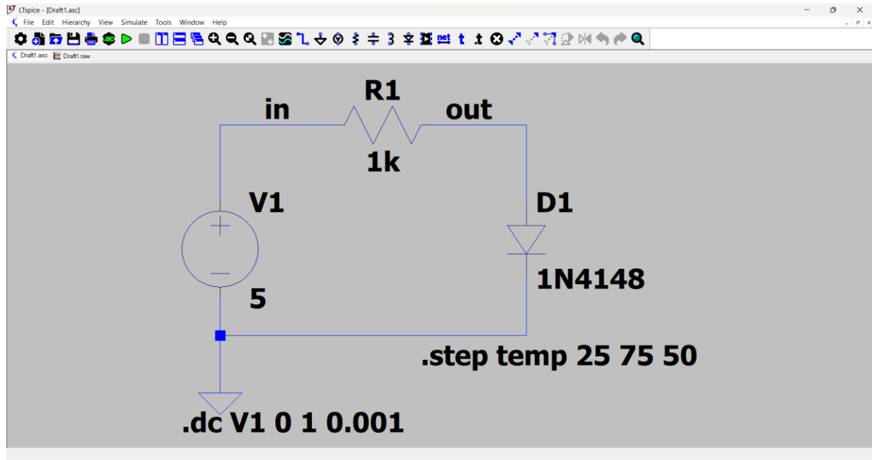
Figure 1: Schematic view of Temperature Effects on Diode Behavior
